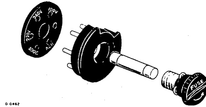
Fig. 7-7 Voltage Conversion
