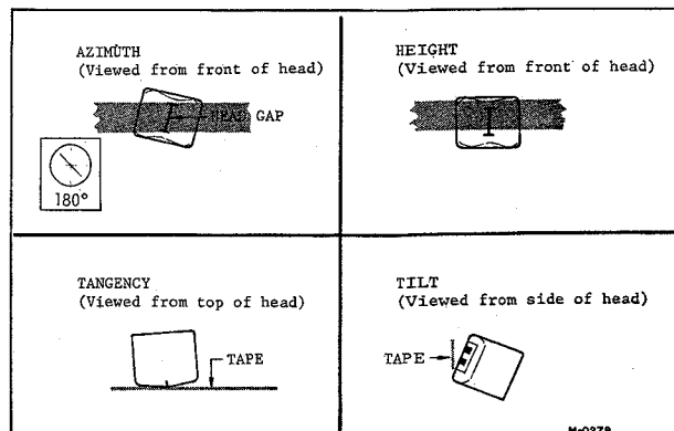
Fig. 6-4 Head Mis-Alignment — Examples —
