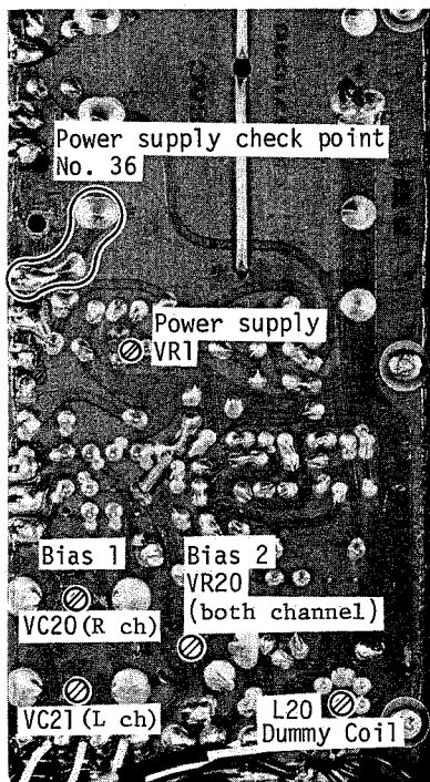
Fig. 9-2 BIAS OSC P.C.B. Adj. Location
